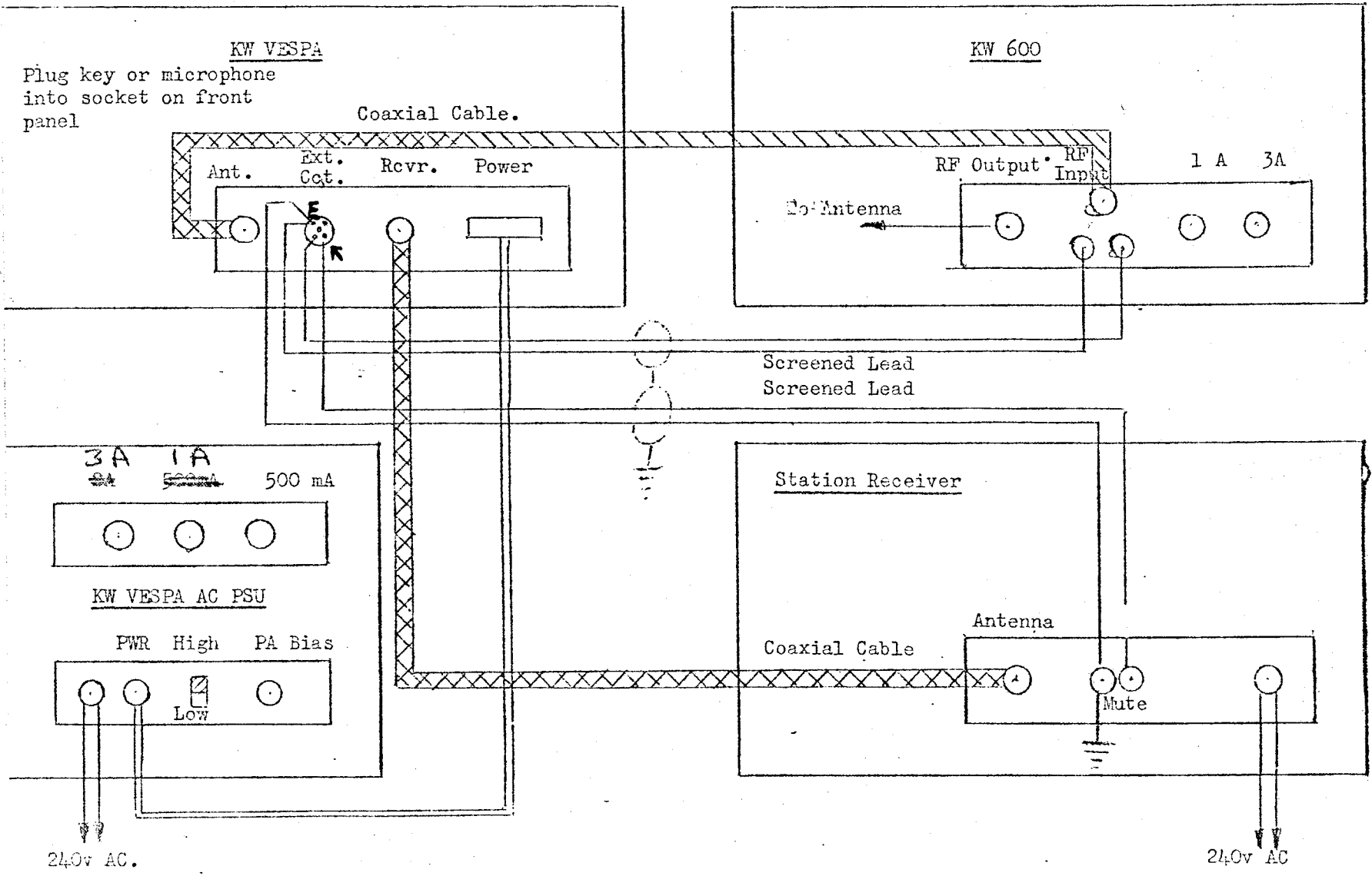
Installation with KW 600
