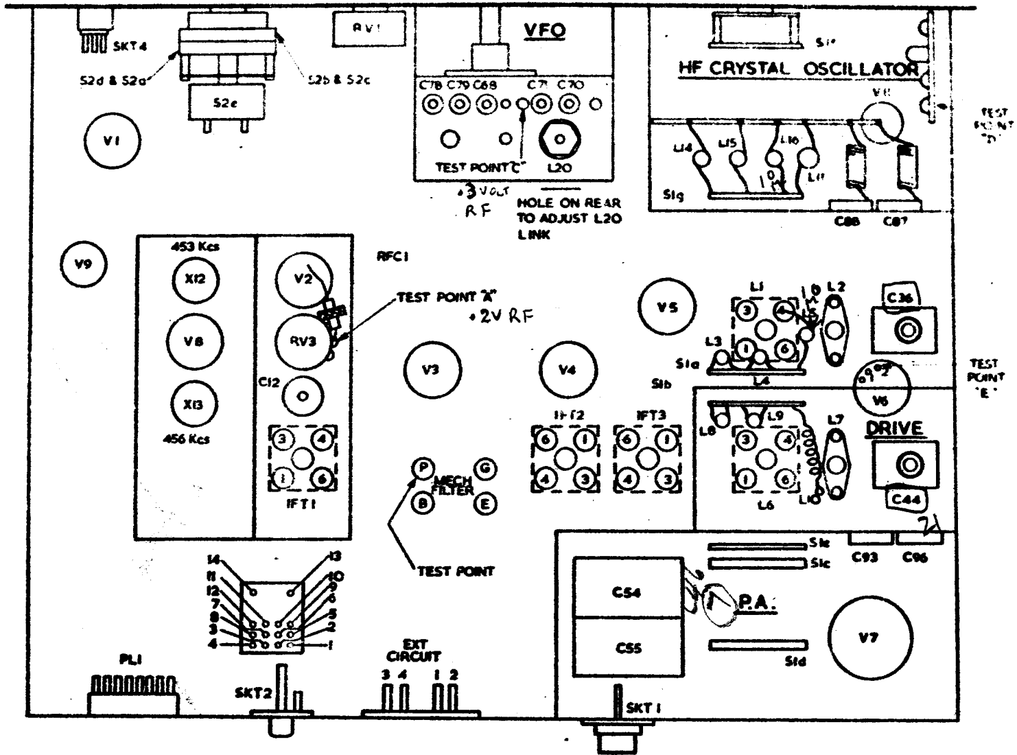
FIG 5-1 LOCATION OF ADJUSTMENTS.
