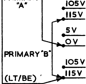
PRIMARY WINDING CONNECTIONS FOR 115V. A.C. OPERATION.
